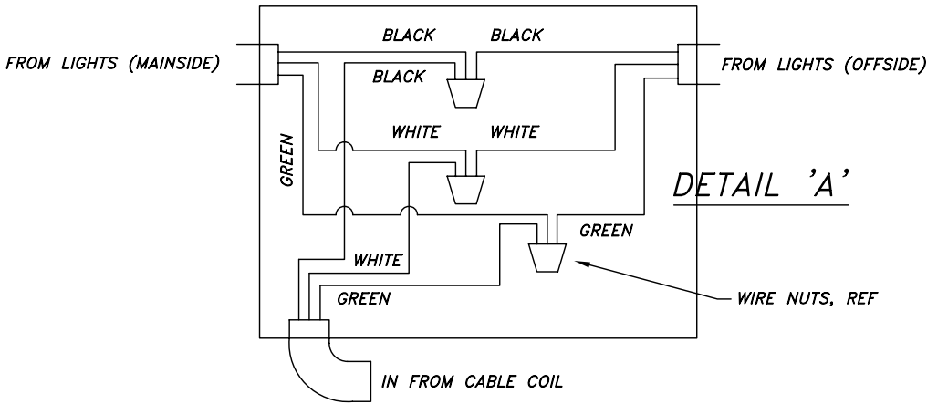
CROSSRAIL JUNCTION BOX WIRING (CONNECT ALL LIKE COLORS TOGETHER)
