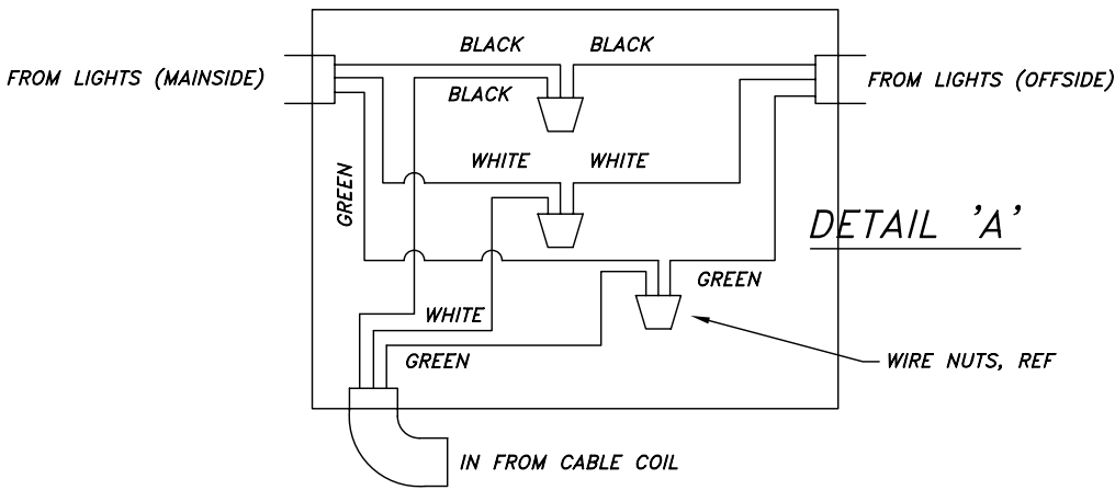
CROSSRAIL JUNCTION BOX WIRING (CONNECT ALL LIKE COLORS TOGETHER)
