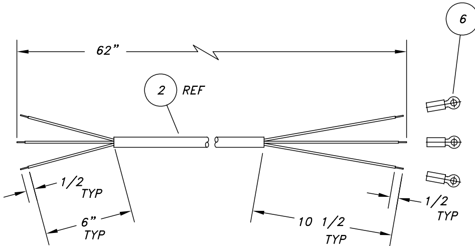
CONDUCTOR STRIPPING DETAIL
