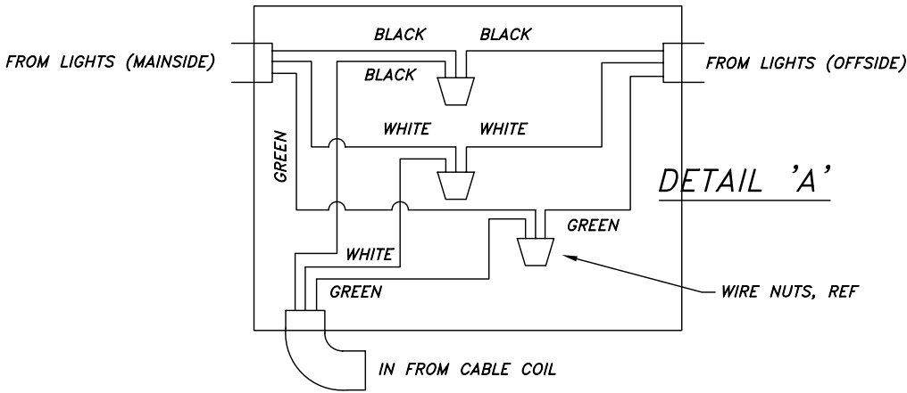
CROSSRAIL JUNCTION
