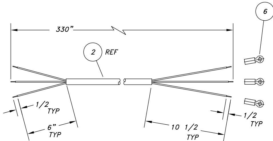
CONDUCTOR STRIPPING DETAIL
