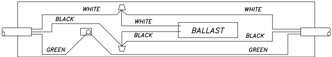
DETAIL 'B' LIGHT FIXTURE WIRING, TYP (CONNECT ALL LIKE COLORS TOGETHER)
